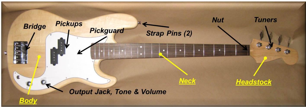
Fig 1 Major Components in Your P Bass Guitar Kit
